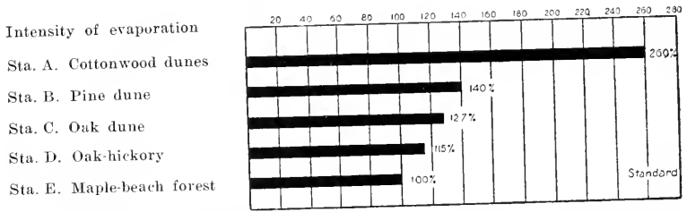
FIG. 5. Diagram showing the relative rate of evaporation in different kinds of forest in northern Illinois and Indiana. [Data from Fuller ('11) and McNutt and Fuller ('12).]
